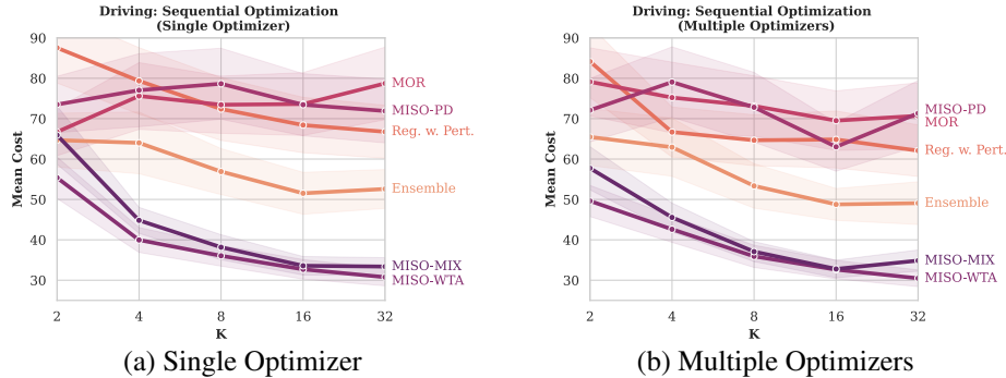
Figure 4: Mean Cost of the autonomous driving environment with varying values of K . The shaded regions around each curve indicate the standard error of the mean.
