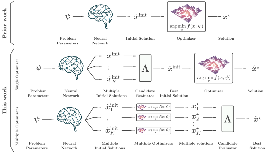
Figure 1: As opposed to previous works that predict a single initial solution, MISO trains a single neural network to predict multiple initial solutions. We use them to either initialize a single optimizer or jointly initialize multiple optimizers.
