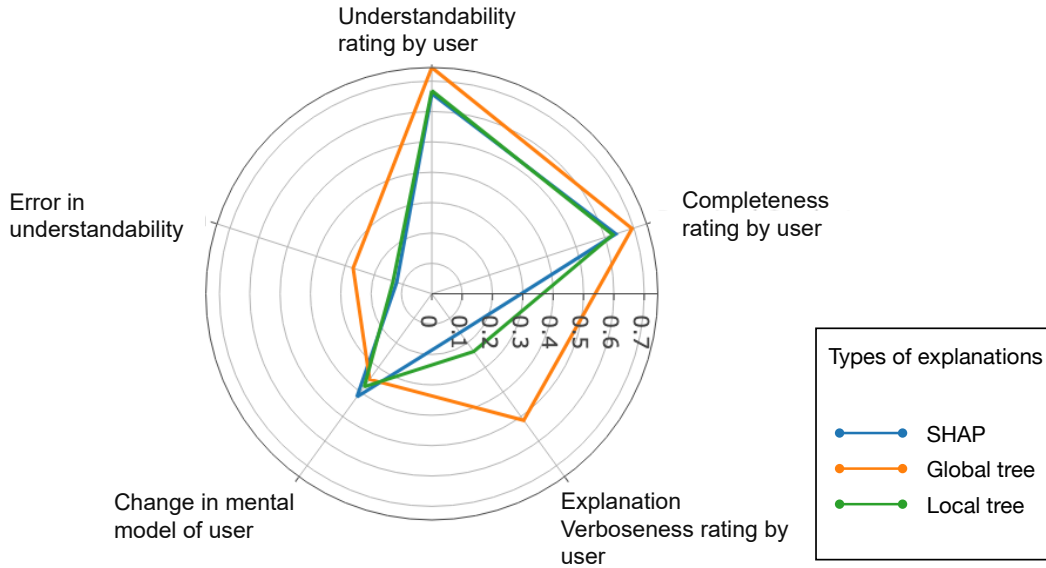
Fig. 1: A comparison of Local SHAP, Local and Global tree explanation of CHD risk prediction using decision tree model. Different evaluation parameters are computed based on end-user feedback of the explanation.
