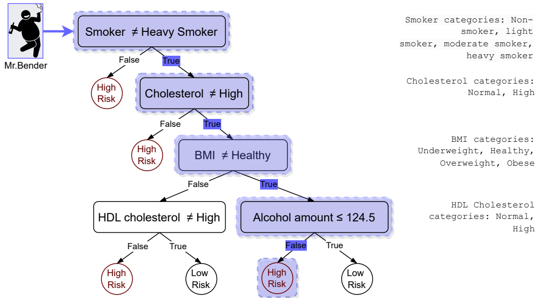
(a) The decision path followed along a given DT for a particular patient Mr Bender. The tree is learned from different categorical features of a patient dataset and the black square boxes represent decision nodes learned by the model. On the right, all the possible values of each feature are listed (except Alcohol amount which is numeric). This tree has 6 leaf nodes each a possible decision of high or low risk . For a given input corresponding to Mr Bender, the model predicts high risk following the decision path highlighted in Blue.
